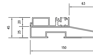
Low Threshold with 150mm Cill
