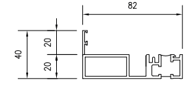
Low Threshold with Rebate - No Cill
