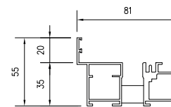
Standard Threshold - No Cill
