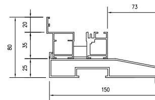
Standard Threshold with 150mm Cill
