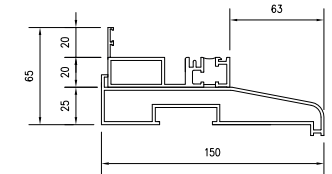
Low Threshold with Rebate & 150mm Cill
